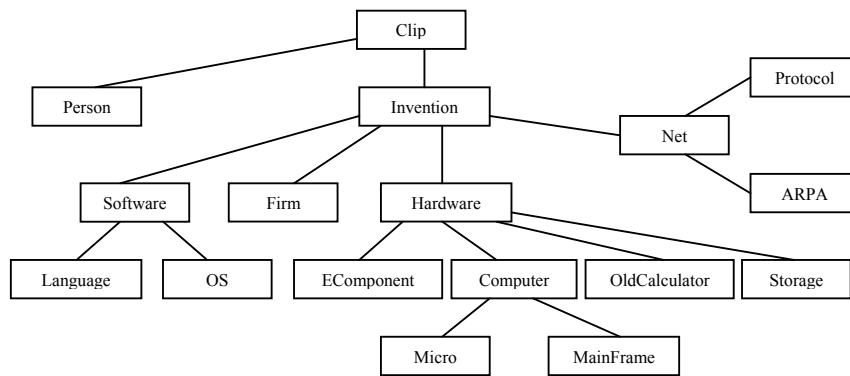
Fig. 2. Class hierarchy of the CHESt RDF classes
